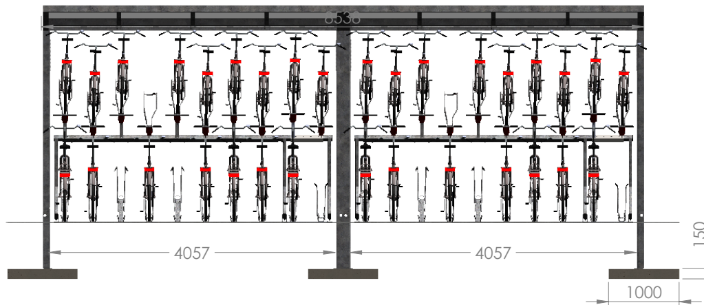
T-Hide single-sided 2 sections - h.2.h. 400 mm
